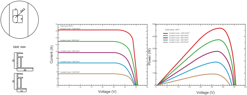
Current-Voltage & Power-Voltage Curves (SKT460M10-120D5)
