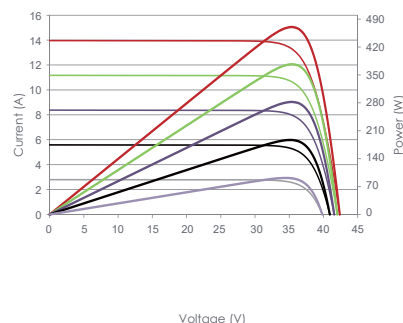
Current-Voltage & Power-Voltage Curves (450W)
