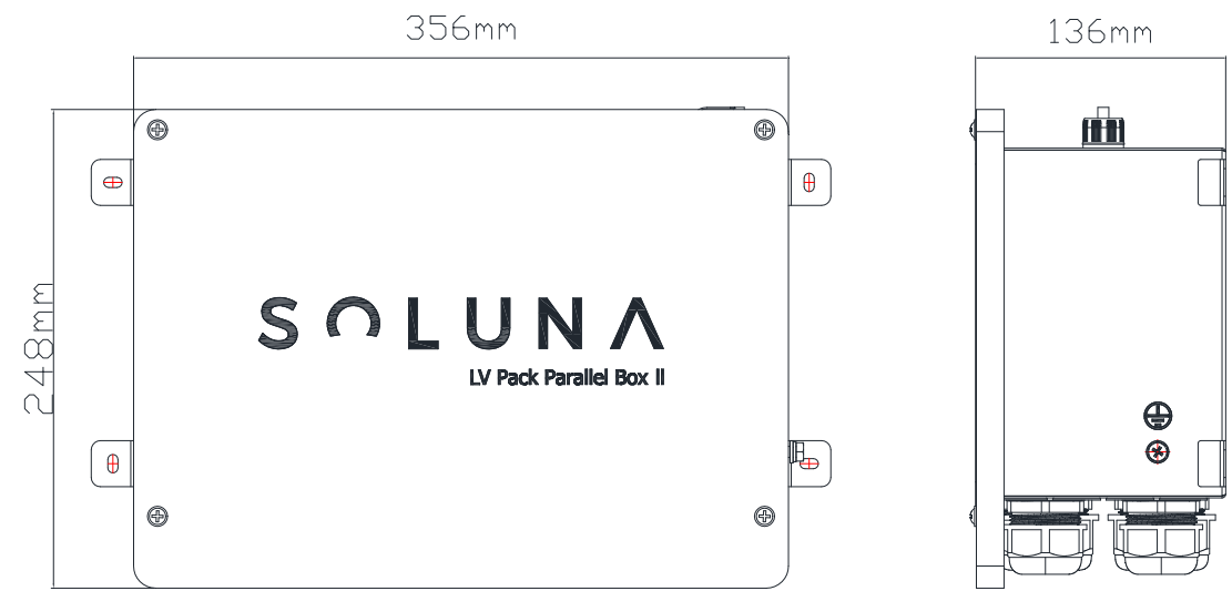
Figure 1.1 outline dimension
